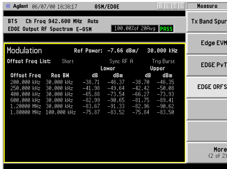
Output RF Spectrum Result (Short List) Modulation View
